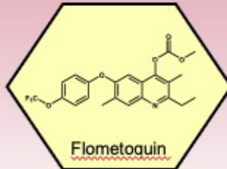
34 Flometoquin
